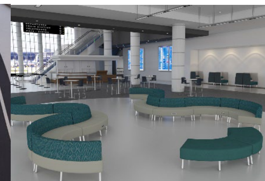
Krug – Zola
